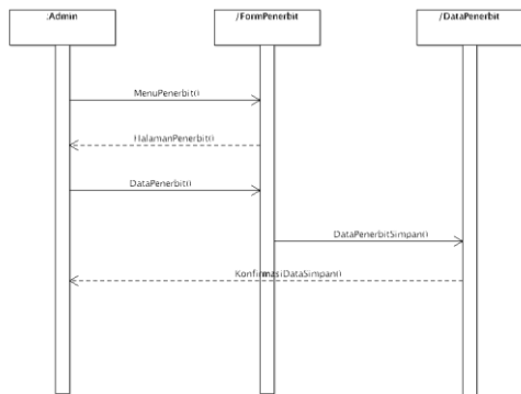
Sequence Diagram Master Admin
