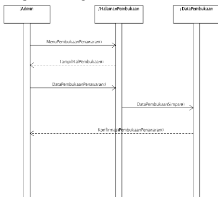
Sequence Diagram Penawaran Supplier
