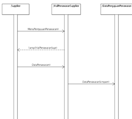
Sequence Diagram Penawaran Supplier
