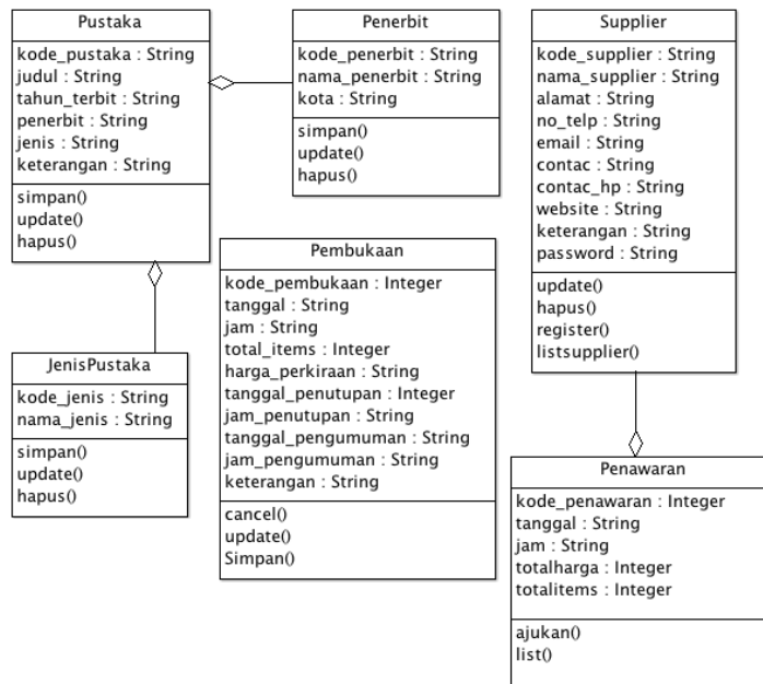
Gambar 5. Class Diagram
